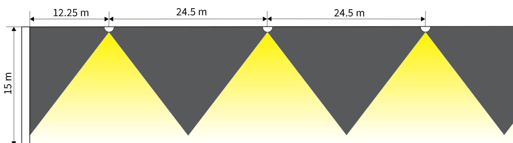
N89-C (1 lx, Centreline), Ceiling Height 15 m
