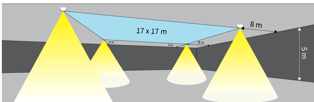
N68-O Hi-Power (0.5 lx, Evac. Area), Ceiling Height 5 m
