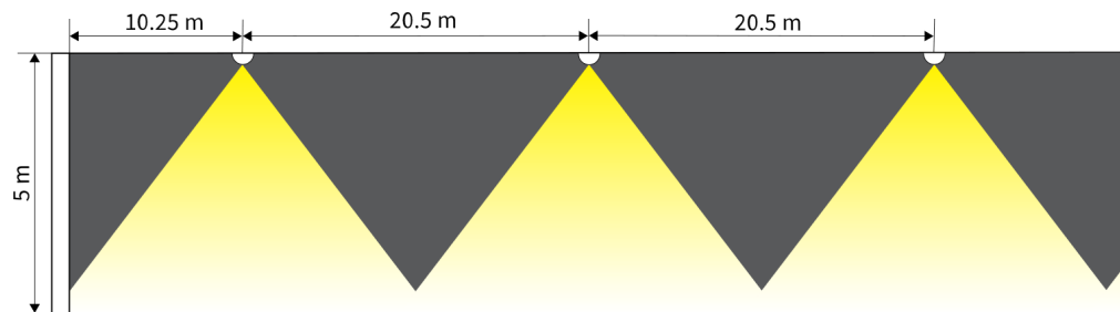
N68-C (0,5 lx, Centreline), Ceiling Height 5 m
