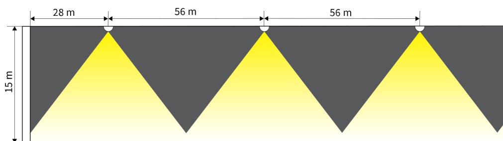
N89-C (0.5 lx, Centreline), Ceiling Height 15 m
