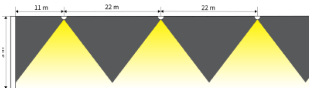
N68-C Hi-Power (1 lx, Centreline), Ceiling Height 5 m
