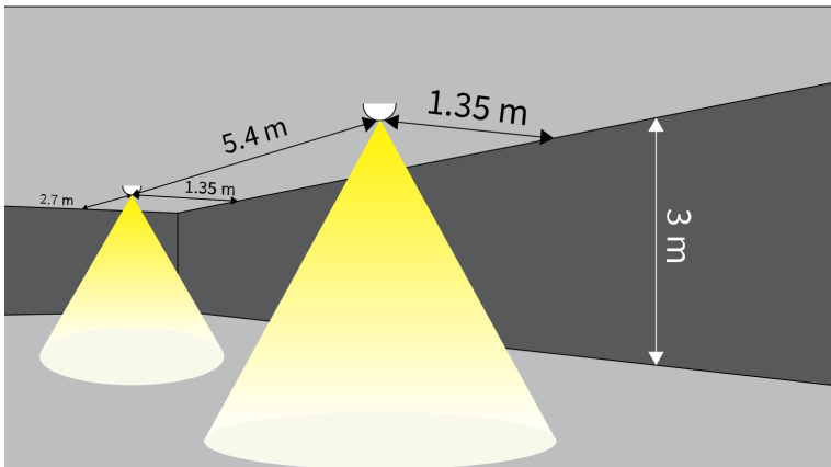
N68-C (5 lx, Centreline), Ceiling Height 3 m
