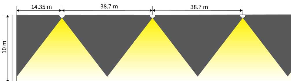
N68-C Hi-Power (0.5 lx, Centreline), Ceiling Height 10 m
