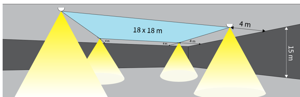
N89-O (0,5 lx, Evac. Area), Ceiling Height 15 m
