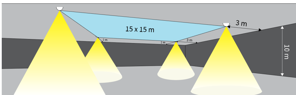
N68-O Hi-Power (0.5 lx, Evac. Area), Ceiling Height 10 m
