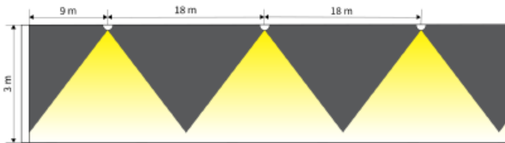
N68-C (0,5 lx, Centreline), Ceiling Height 3 m
