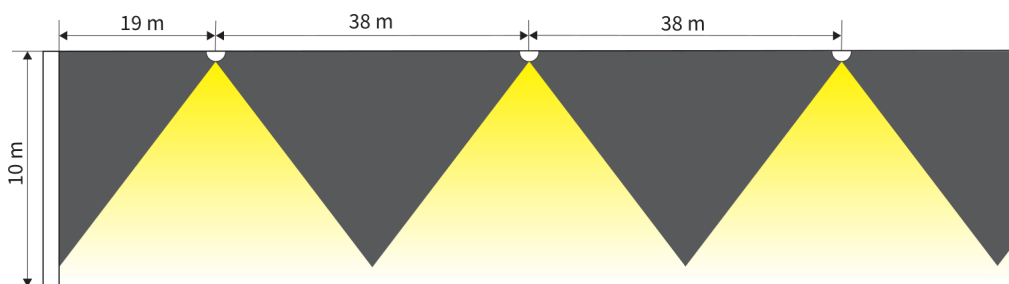
N89-C (1 lx, Centreline), Ceiling Height 10 m
