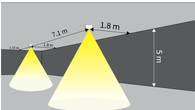
N68-C Hi-Power (5 lx, Centreline), Ceiling Height 5 m
