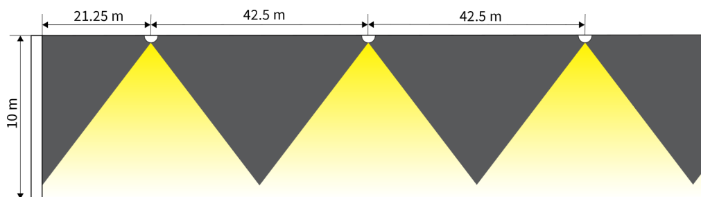
N89-C (0.5 lx, Centreline), Ceiling Height 10 m
