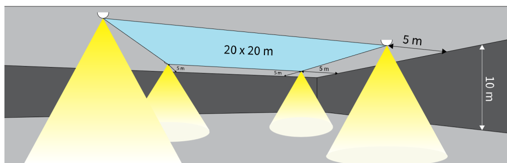
N89-O (0,5 lx, Evac. Area), Ceiling Height 10 m
