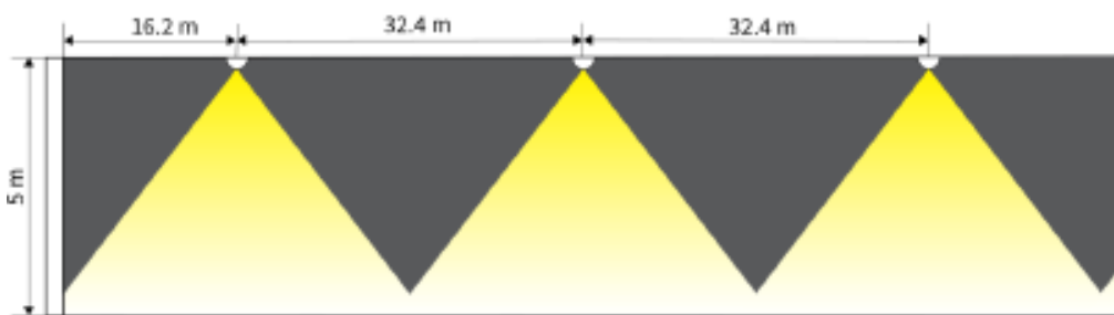
N68-C Hi-Power (0.5 lx, Centreline), Ceiling Height 5 m
