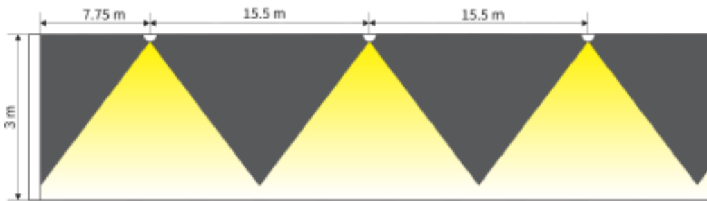
N68-C (1 lx, Centreline), Ceiling Height 3 m
