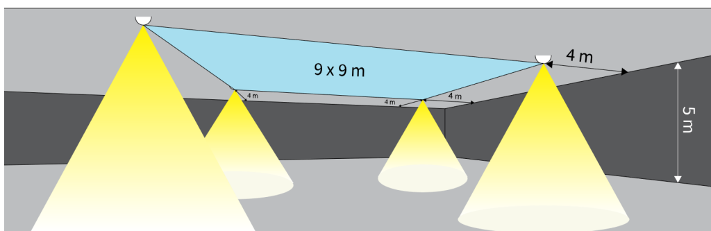
N68-O (0.5 lx, Evac. Area), Ceiling Height 5 m
