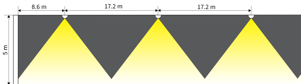
N89-C (5 lx, Centreline), Ceiling Height 5 m
