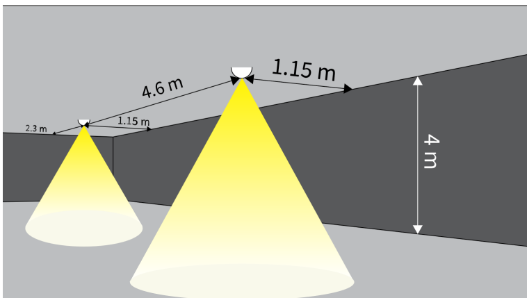
N68-C (5 lx, Centreline), Ceiling Height 4 m
