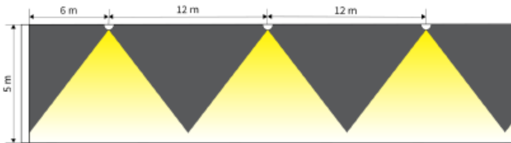
N68-C (1 lx, Centreline), Ceiling Height 5 m
