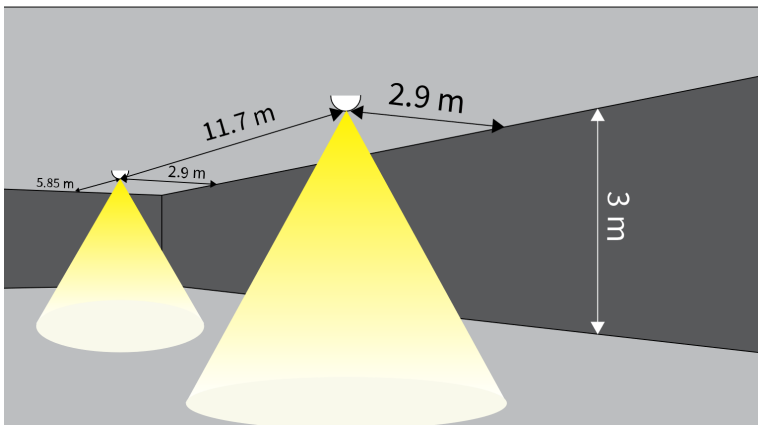
N68-C Hi-Power (5 lx, Centreline), Ceiling Height 3 m
