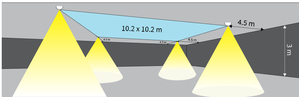
N68-O (0.5 lx, Evac. Area), Ceiling Height 3 m
