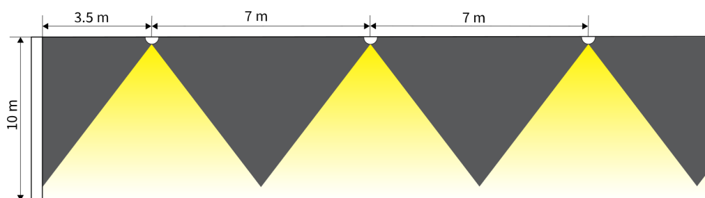
N89-C (5 lx, Centreline), Ceiling Height 10 m
