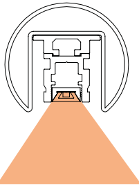
Symmetrical Handrail 48.3 with Top LED strip Product code: 12049
