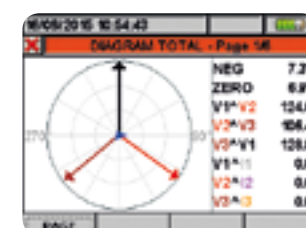
Voltage and current vector diagram
