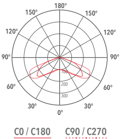
Perimetral lighting
