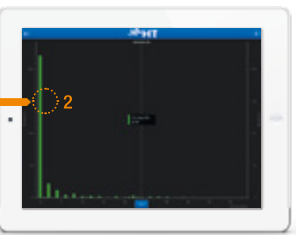
Jump Function
